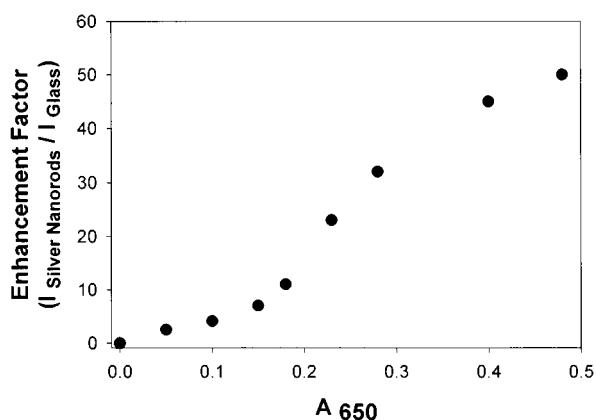
Fig. 23. Fluorescence emission intensity of HSA-ICG on silver nanorods (top) and enhancement factor vs the absorption of silver nanorods measured at 650 nm.
