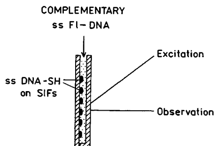
Fig. 15. Time-dependent hybridization of ss FI-DNA to ss DNA-SH. The lower panel shows the sample configuration.
